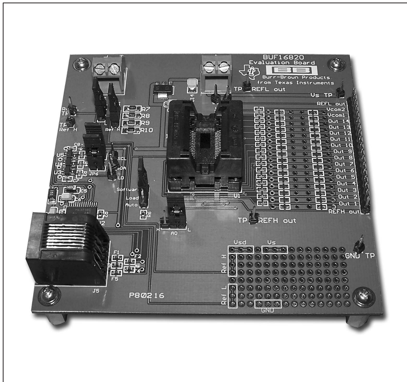
Figure 21. Evaluation Board
